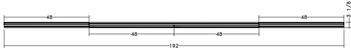
2 A SECTION 3/8" = 1'-0"
