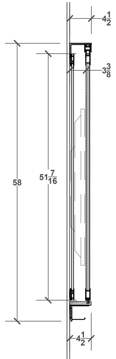
4 Enlarged Section 1" = 1'-0"
