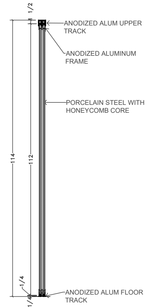
3 A SECTION 1/2" = 1'-0"
